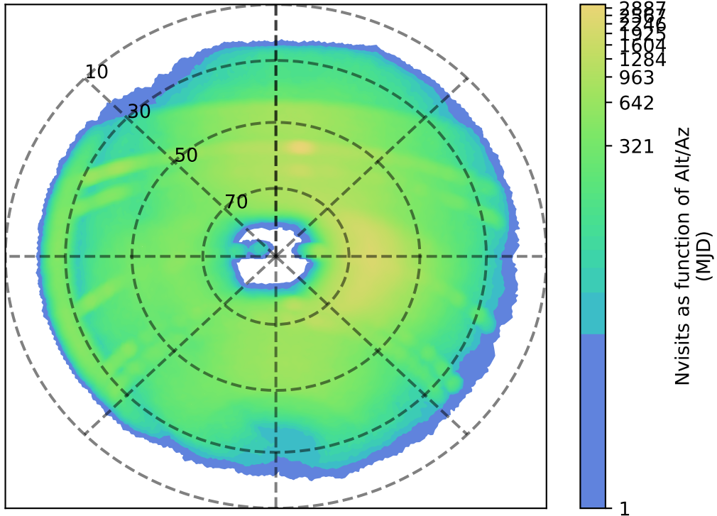
ddf_acor_sf10_ls40_lsr50_v3.4_10yrs r: Nvisits as function of Alt/Az
