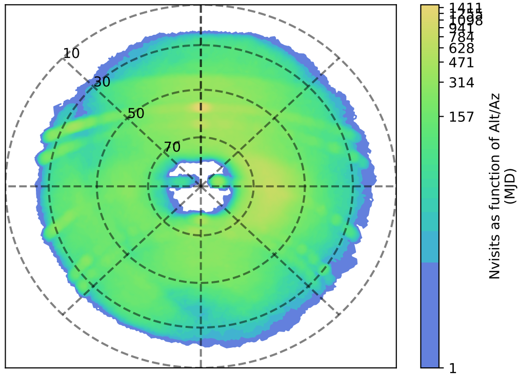
ddf_acor_sf10_lsf40_lsr50_v3.4_10yrs g: Nvisits as function of Alt/Az
