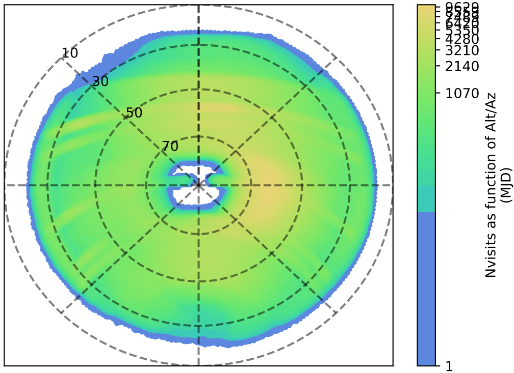
ddf_acor_sf10_lsf40_lsr50_v3.4_10yrs : Nvisits as function of Alt/Az
