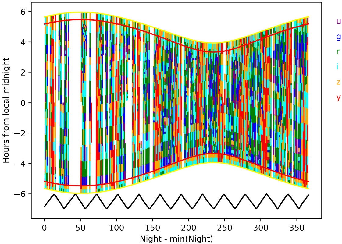
ddf_acor_sf10_lsf40_lsr50_v3.4_10yrs year 8-9: Hourglass
