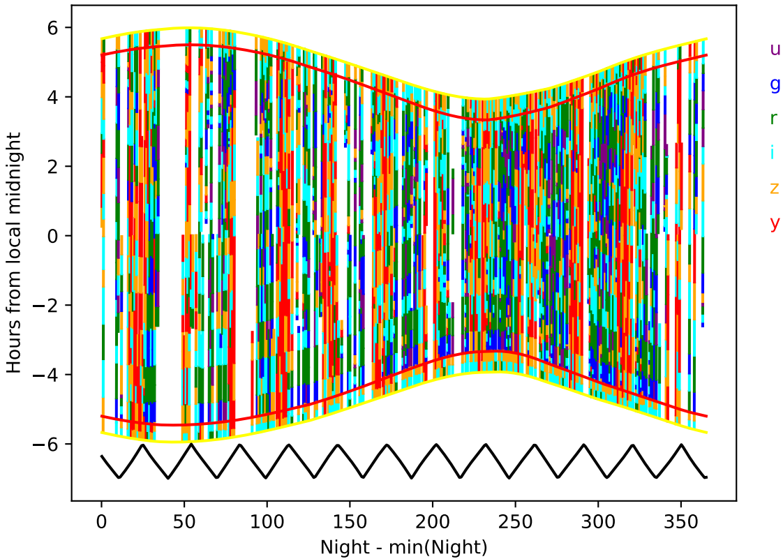
ddf_acor_sf10_lsf40_lsr50_v3.4_10yrs year 4-5: Hourglass
