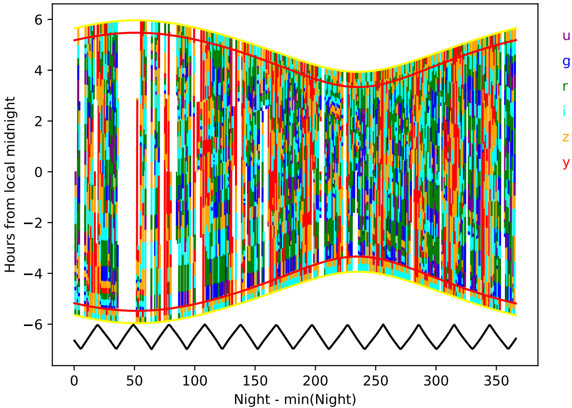
ddf_acor_sf10_lsf40_lsr50_v3.4_10yrs year 2-3: Hourglass
