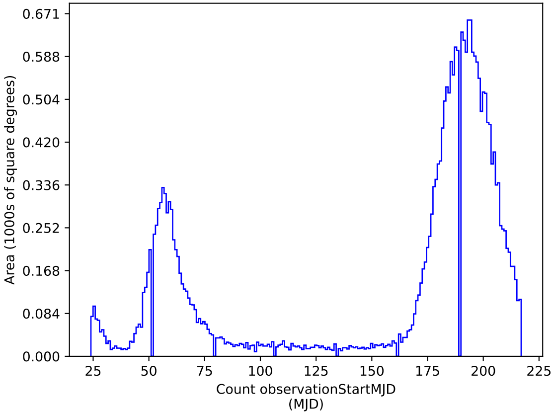
ddf_acor_sf10_lsf40_lsr50_v3.4_10yrs i: Count observationStartMJD
