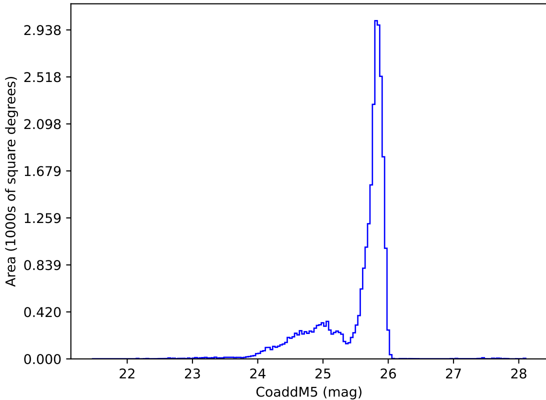
ddf_acor_sf10_lsf40_lsr50_v3.4_10yrs z: CoaddM5
