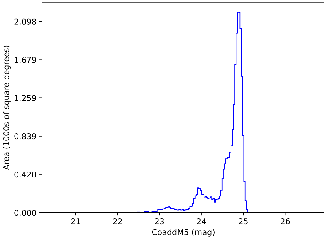
ddf_acor_sf10_lsf40_lsr50_v3.4_10yrs y: CoaddM5
