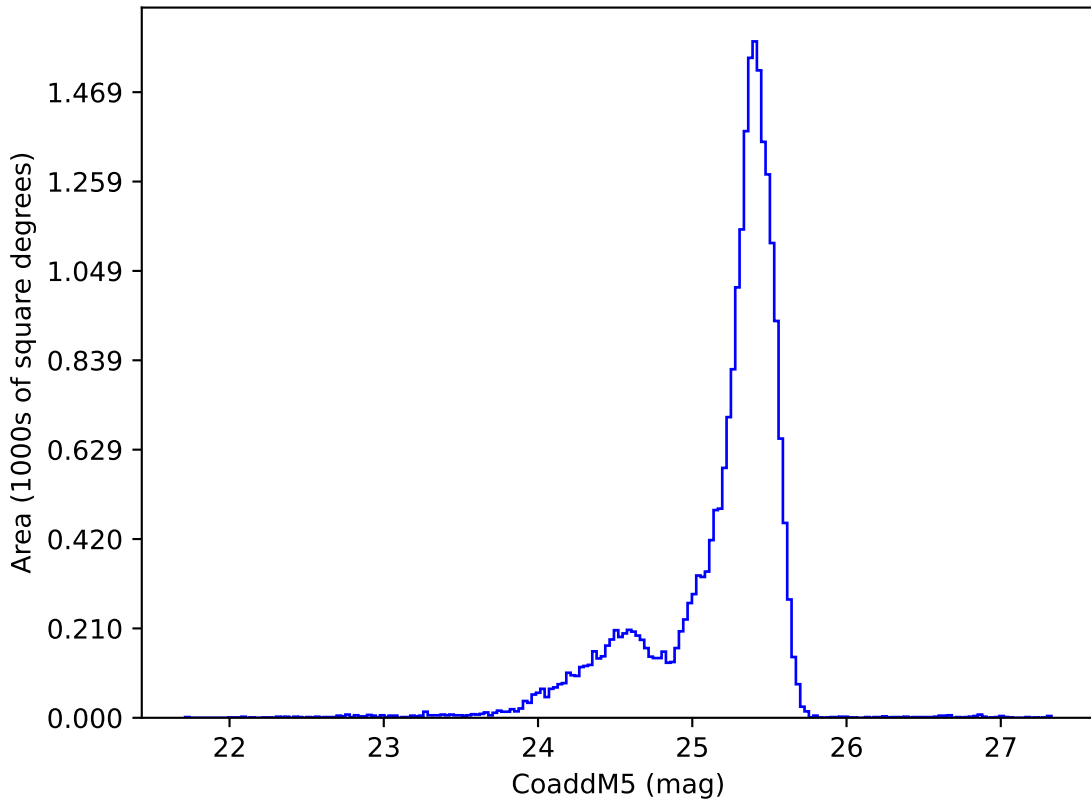
ddf_acor_sf10_lsf40_lsr50_v3.4_10yrs u: CoaddM5
