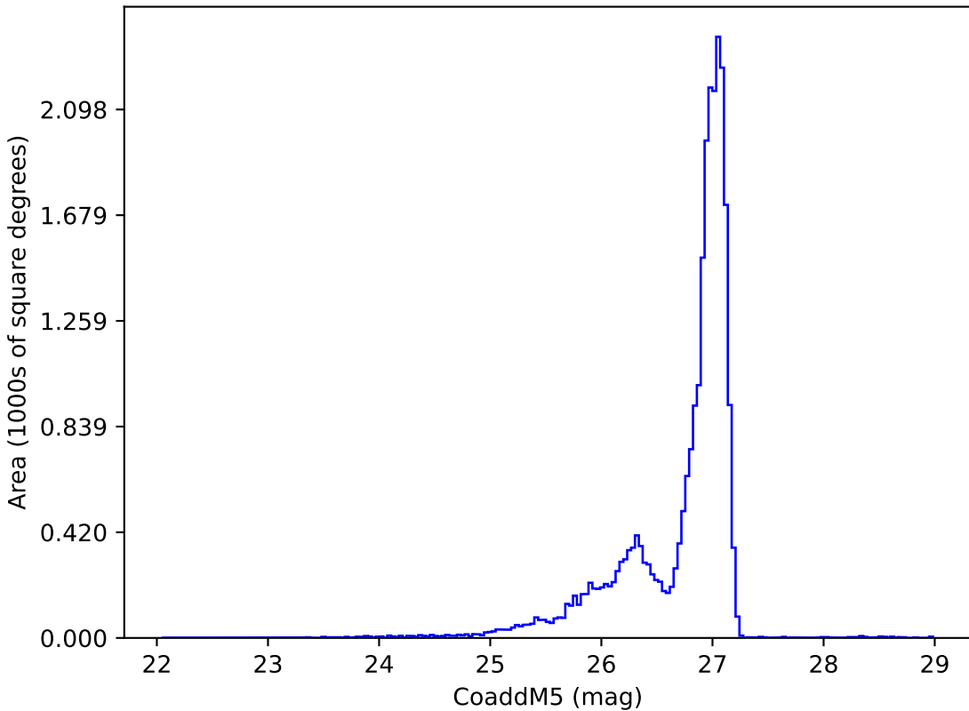
ddf_acor_sf10_lsf40_lsr50_v3.4_10yrs r: CoaddM5
