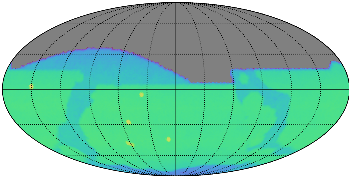
ddf_acor_sf10_lsf40_lsr50_v3.4_10yrs i: CoaddM5
