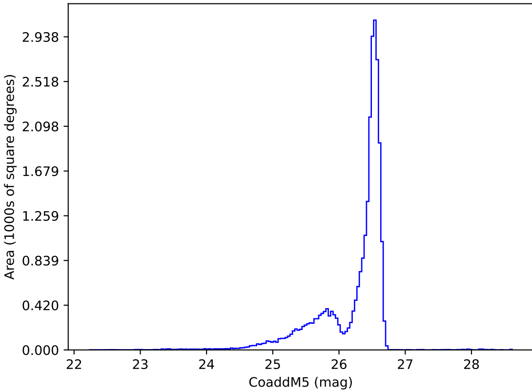
ddf_acor_sf10_lsf40_lsr50_v3.4_10yrs i: CoaddM5
