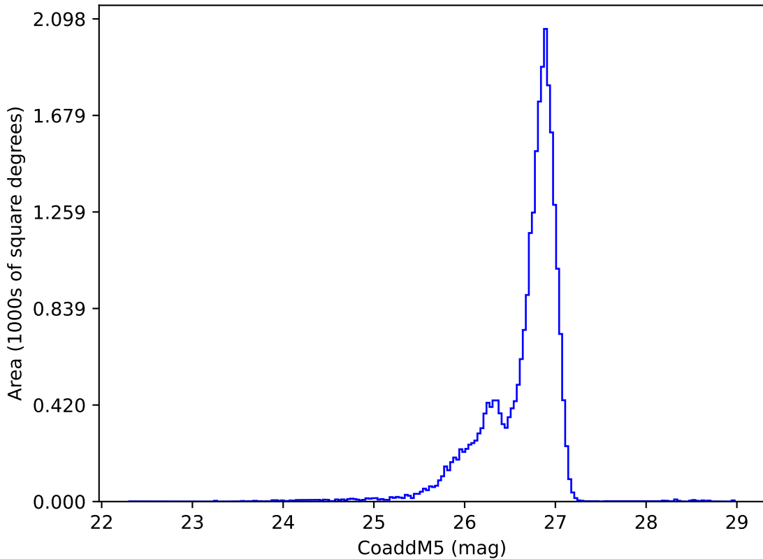
ddf_acor_sf10_ls40_lsr50_v3.4_10yrs g: CoaddM5
