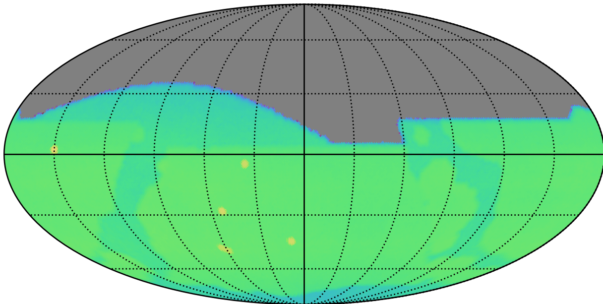
ddf_acor_sf10_lsf40_lsr50_v3.4_10yrs : CoaddM5
