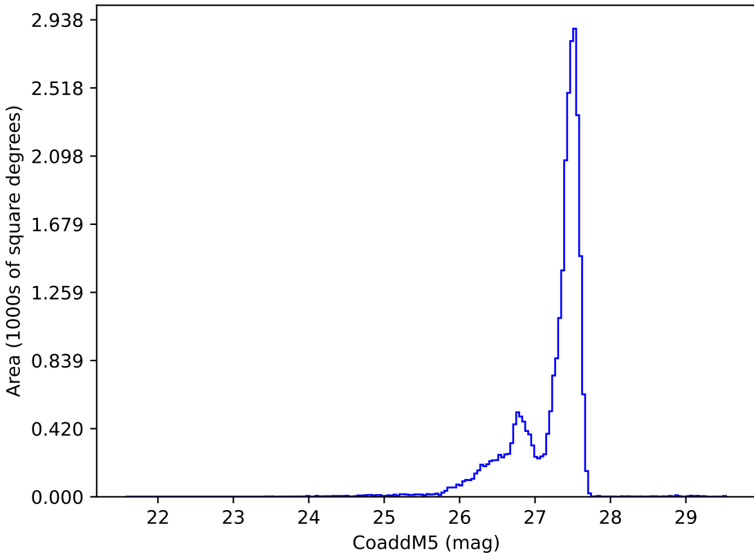
ddf_acor_sf10_lsf40_lsr50_v3.4_10yrs : CoaddM5
