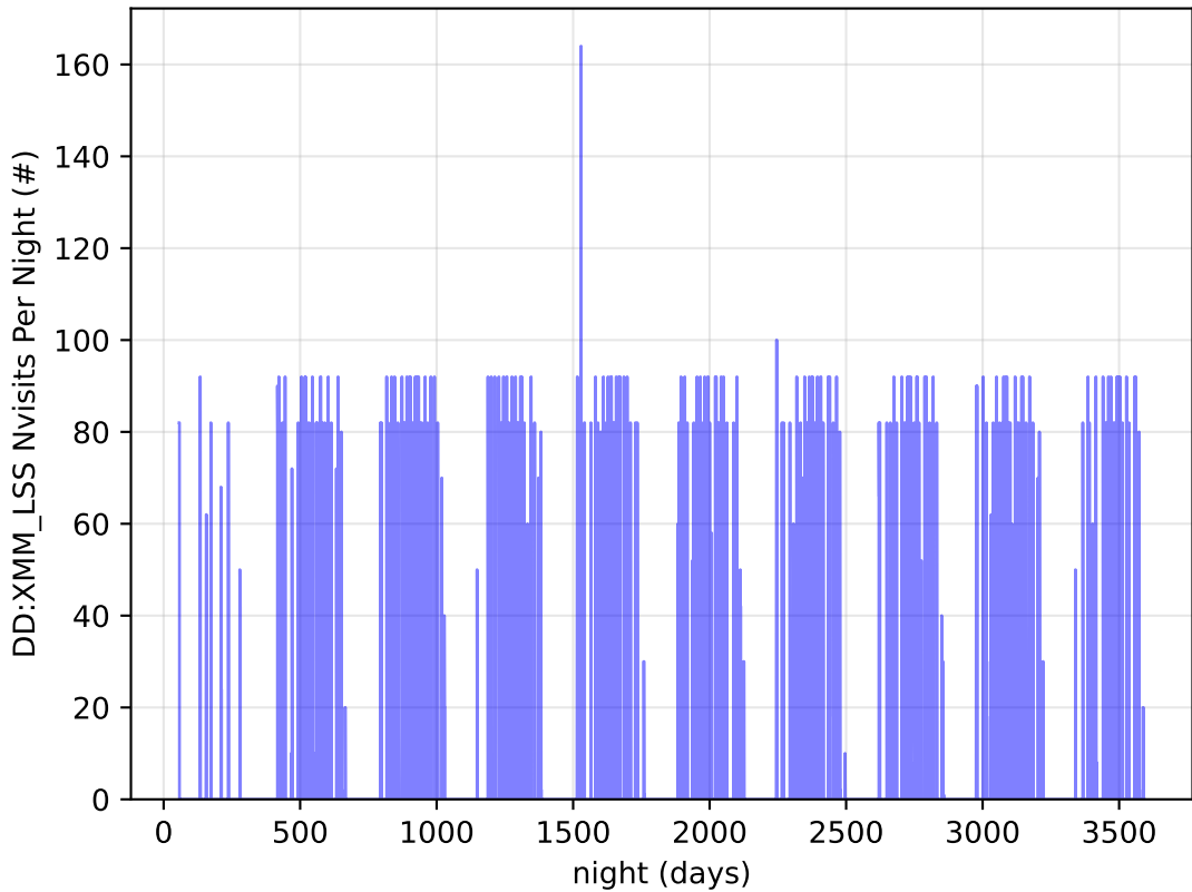
ddf_acor_sf10_lsf40_lsr50_v3.4_10yrs all bands: DD:XMM_LSS Nvisits Per Night
