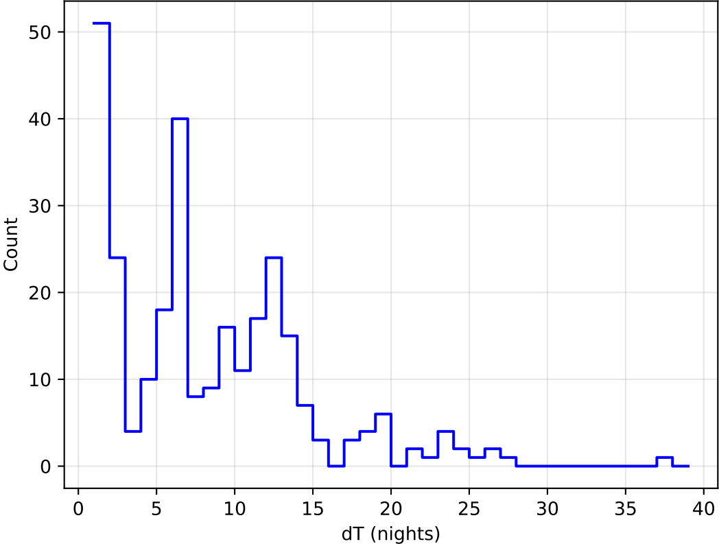
ddf_acor_sf10_lsf40_lsr50_v3.4_10yrs all bands: DD:XMM_LSS Delta Nights Histogram
