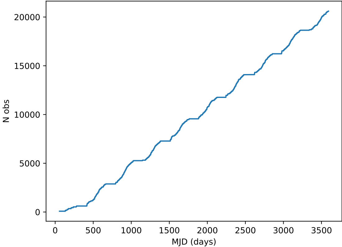
ddf_acor_sf10_lsf40_lsr50_v3.4_10yrs all bands: DD:XMM_LSS Cumulative NVisits
