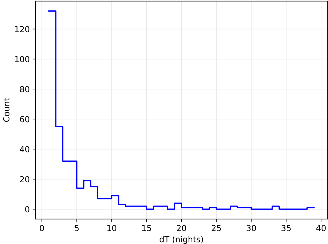
ddf_acor_sf10_lsf40_lsr50_v3.4_10yrs all bands: DD:WFD Delta Nights Histogram
