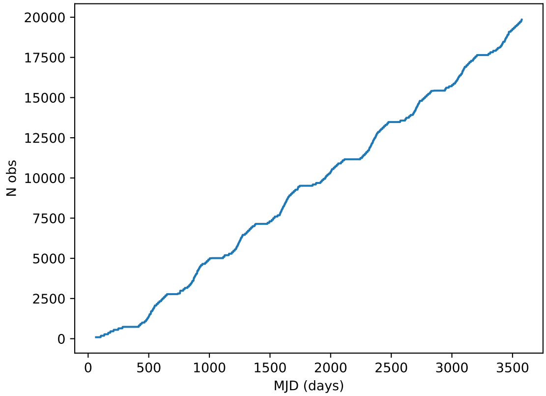
ddf_acor_sf10_lsf40_lsr50_v3.4_10yrs all bands: DD:ELAISS1 Cumulative NVisits
