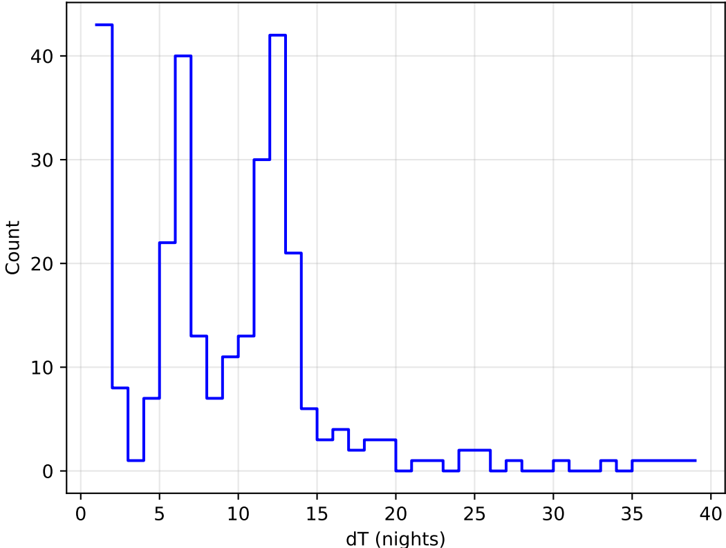
ddf_acor_sf10_Isf40_Isr50_v3.4_10yrs all bands: DD:EDFS Delta Nights Histogram
