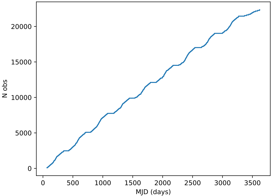
ddf_acor_sf10_lsf40_lsr50_v3.4_10yrs all bands: DD:EDFS Cumulative NVisits
