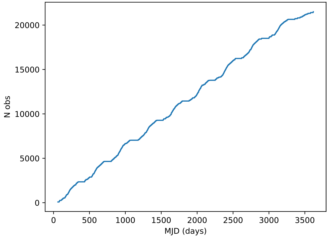
ddf_acor_sf10_lsf40_lsr50_v3.4_10yrs all bands: DD:ECDFS Cumulative NVisits
