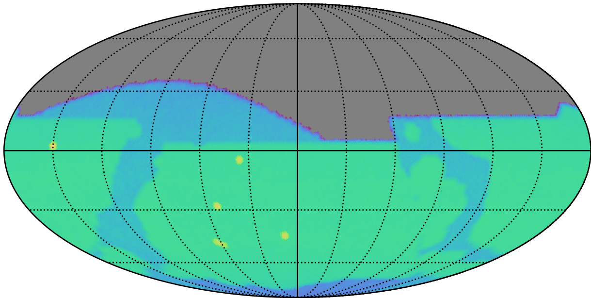
ddf_acor_sf10_lsf40_lsr20_v3.4_10yrs i: SurfaceBrightLimit
