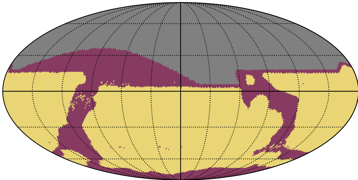
ddf_acor_sf10_lsf40_lsr20_v3.4_10yrs : RapidRevisits
