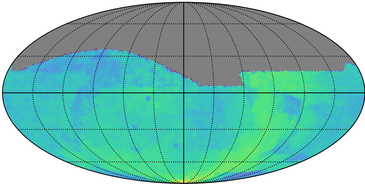
ddf_acor_sf10_lsf40_lsr20_v3.4_10yrs : Parallax Coverage @ 22.4
