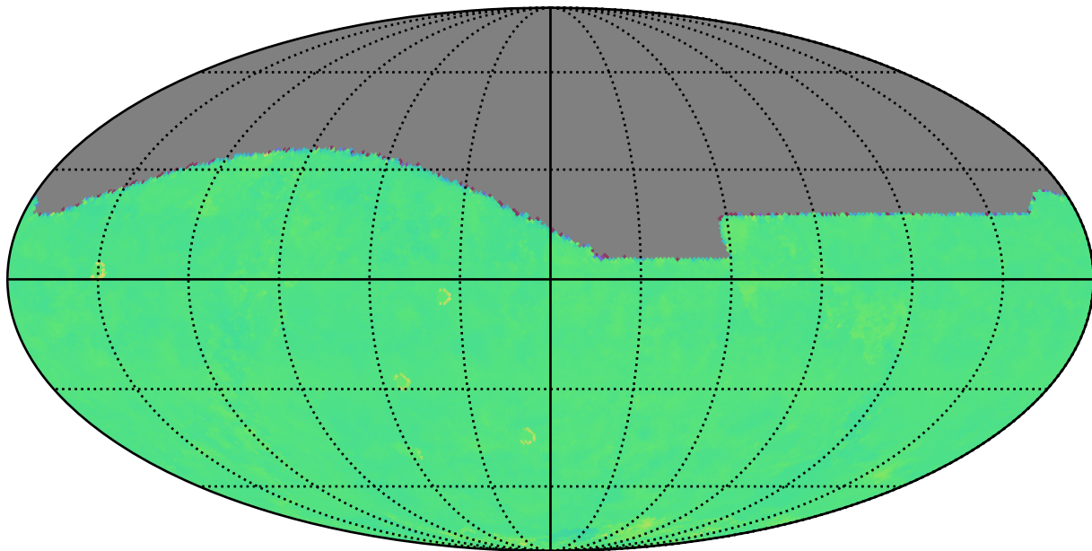
ddf_acor_sf10_lsf40_lsr20_v3.4_10yrs r: Kuiper rotTelPos
