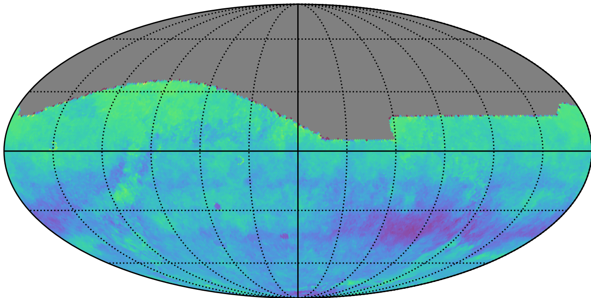
ddf_acor_sf10_lsf40_lsr20_v3.4_10yrs r: Kuiper rotSkyPos
