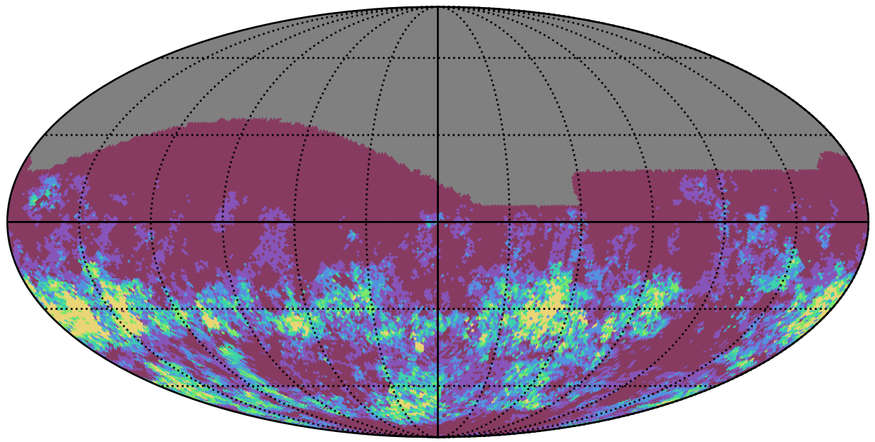
ddf_acor_sf10_lsf40_lsr20_v3.4_10yrs r band: Gaps_7hr
