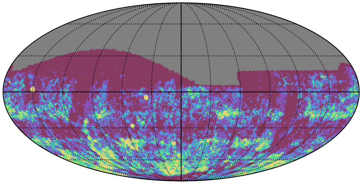
ddf_acor_sf10_lsf40_lsr20_v3.4_10yrs r band: Gaps_3hr
