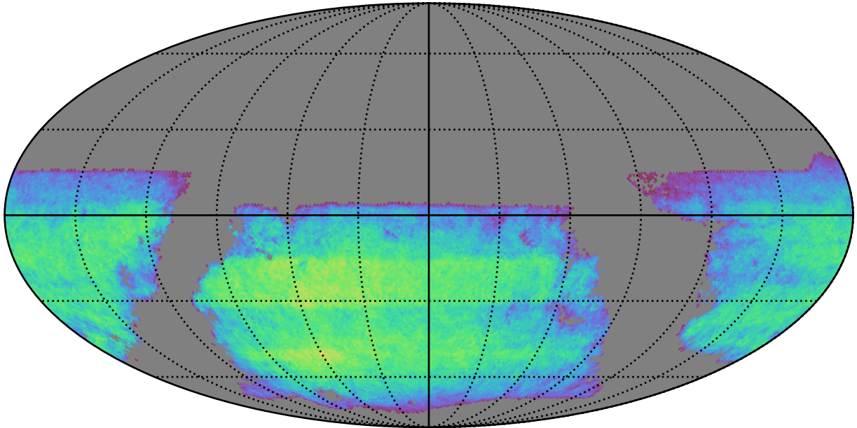
ddf_acor_sf10_lsf40_lsr20_v3.4_10yrs i band non-DD year 7: ExgalM5WithCuts
