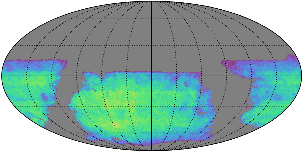
ddf_acor_sf10_lsf40_lsr20_v3.4_10yrs i band non-DD year 4: ExgalM5WithCuts
