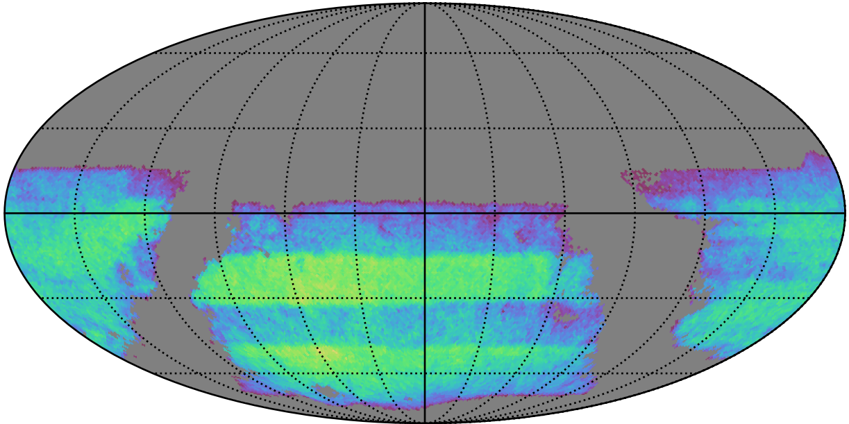
ddf_acor_sf10_lsf40_lsr20_v3.4_10yrs i band non-DD year 3: ExgalM5WithCuts
