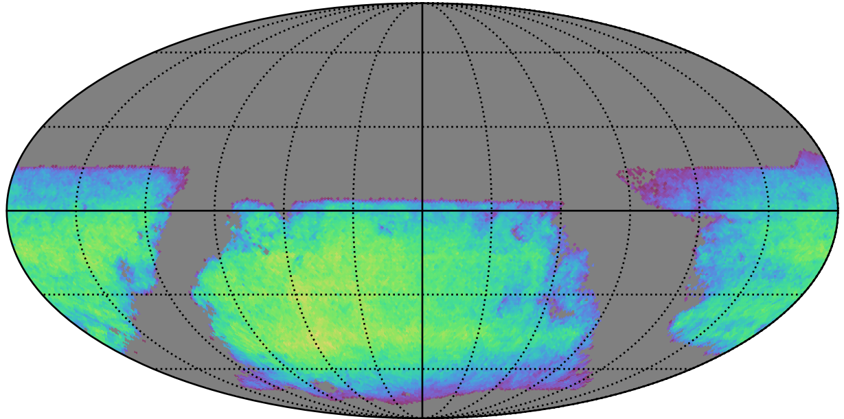
ddf_acor_sf10_lsf40_lsr20_v3.4_10yrs i band non-DD year 10: ExgalM5WithCuts
