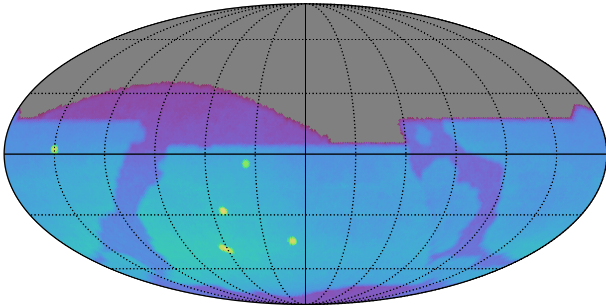
ddf_acor_sf10_lsf40_lsr20_v3.4_10yrs : Brown Dwarf, L4
