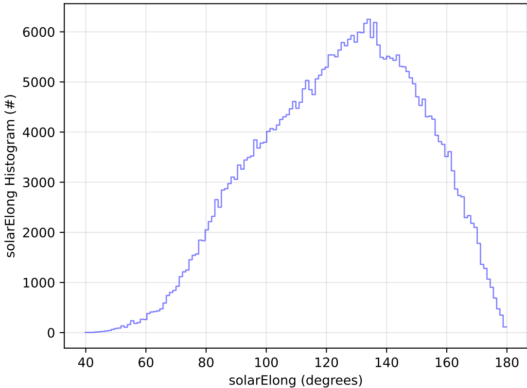
ddf_acor_sf10_lsf40_lsr20_v3.4_10yrs WFD y band: solarElong Histogram
