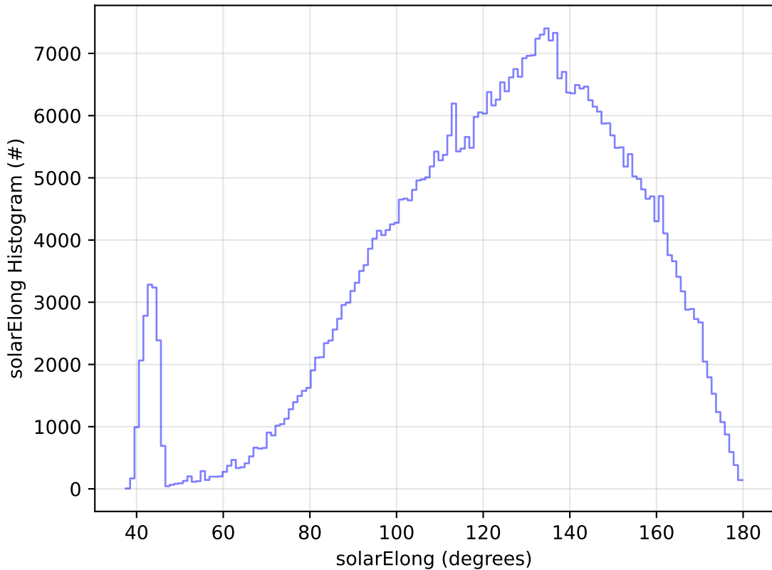
ddf_acor_sf10_ls40_lsr20_v3.4_10yrs WFD r band: solarElong Histogram
