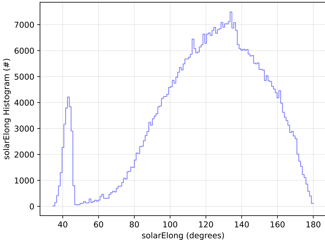
ddf_acor_sf10_lsf40_lsr20_v3.4_10yrs WFD i band: solarElong Histogram
