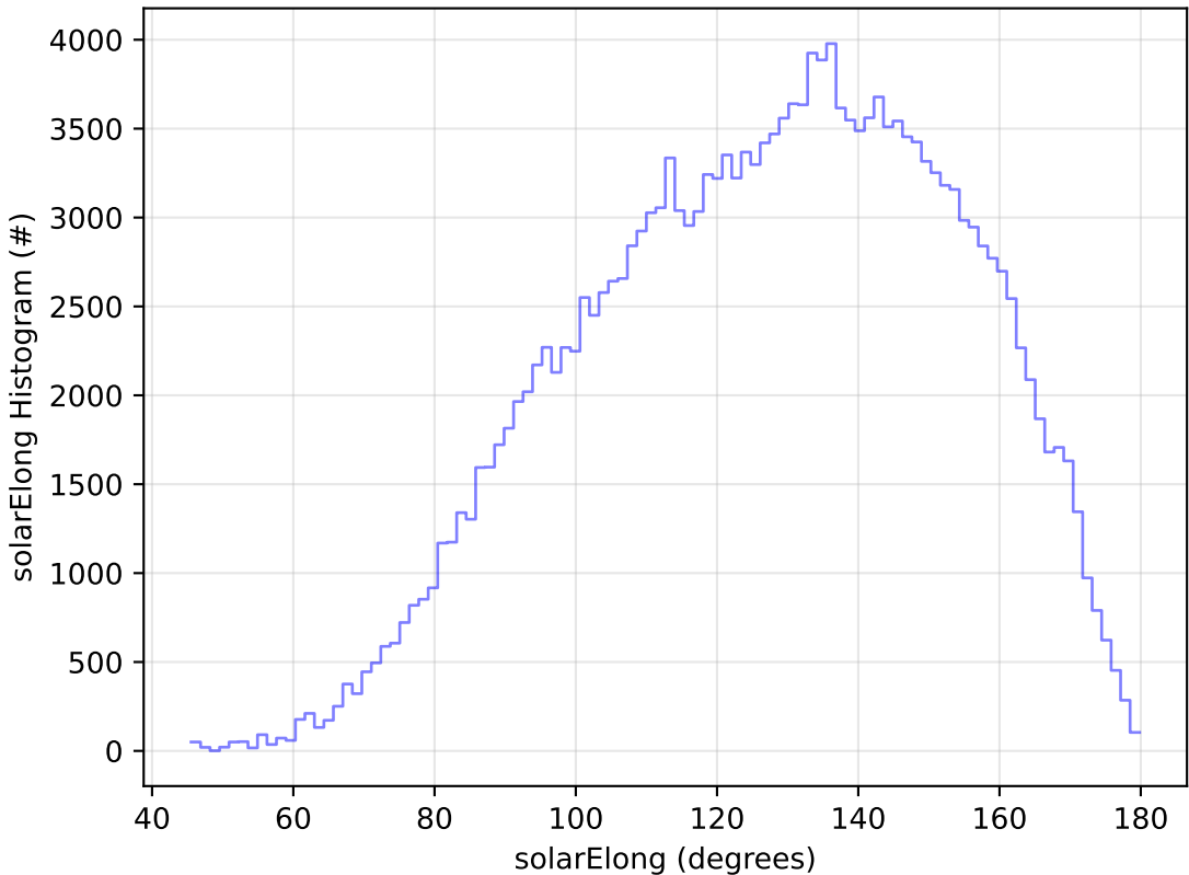
ddf_acor_sf10_lsf40_lsr20_v3.4_10yrs WFD g band: solarElong Histogram
