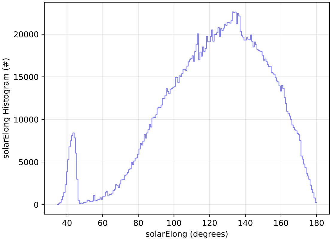
ddf_acor_sf10_lsf40_lsr20_v3.4_10yrs WFD all bands: solarElong Histogram
