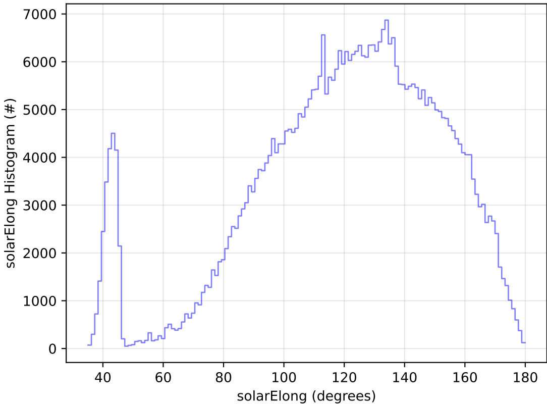
ddf_acor_sf10_lsf40_lsr20_v3.4_10yrs All sky z band: solarElong Histogram
