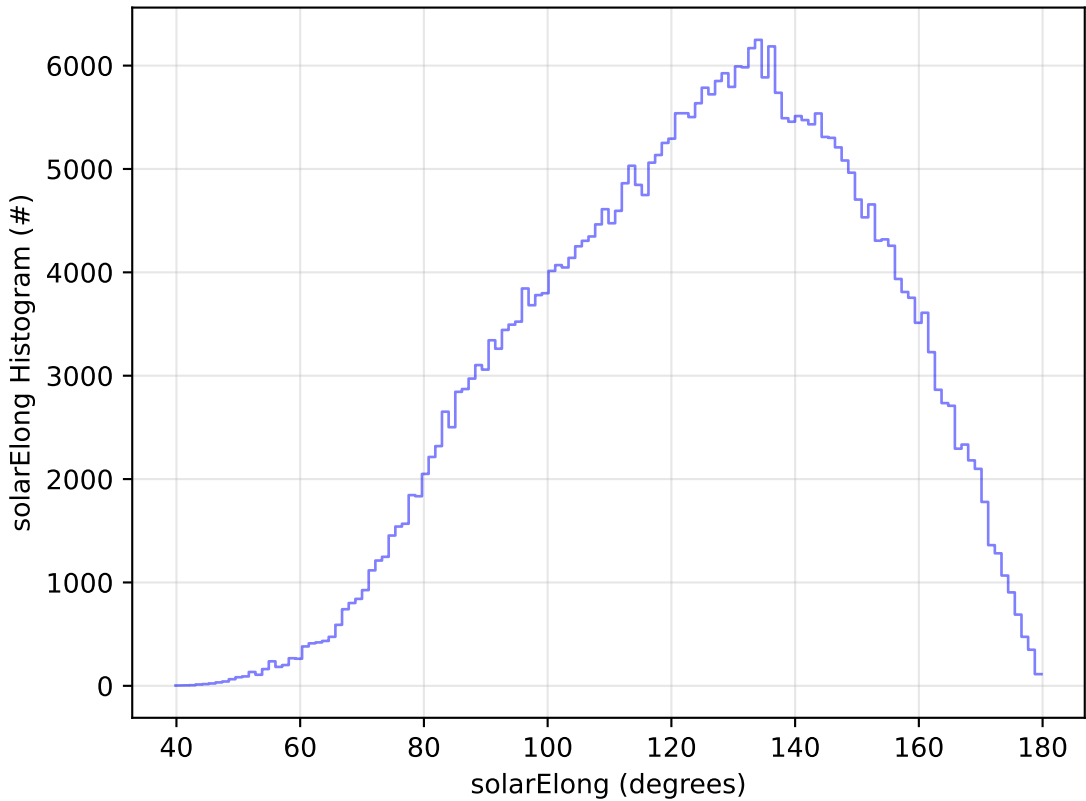
ddf_acor_sf10_lsf40_lsr20_v3.4_10yrs All sky y band: solarElong Histogram
