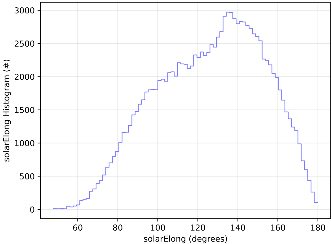
ddf_acor_sf10_lsf40_lsr20_v3.4_10yrs All sky u band: solarElong Histogram
