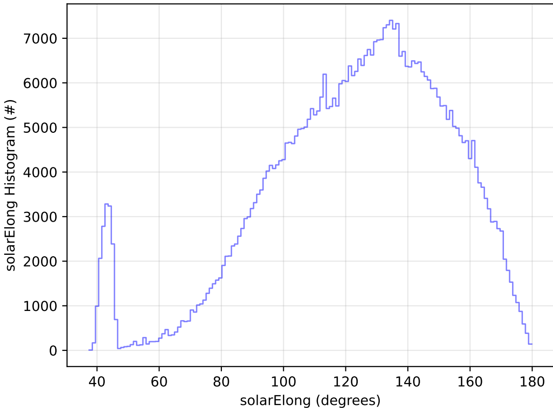
ddf_acor_sf10_lsf40_lsr20_v3.4_10yrs All sky r band: solarElong Histogram
