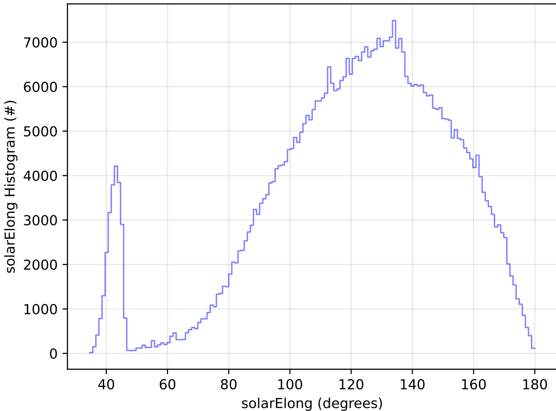
ddf_acor_sf10_lsf40_lsr20_v3.4_10yrs All sky i band: solarElong Histogram
