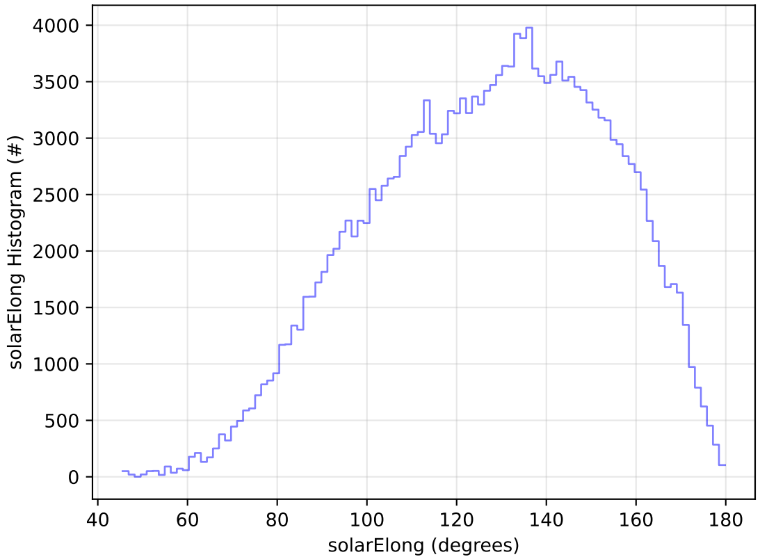
ddf_acor_sf10_lsf40_lsr20_v3.4_10yrs All sky g band: solarElong Histogram
