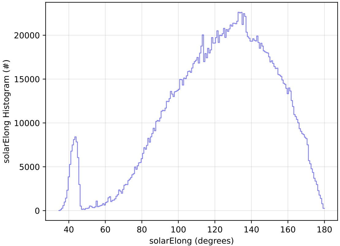
ddf_acor_sf10_lsf40_lsr20_v3.4_10yrs All sky all bands: solarElong Histogram
