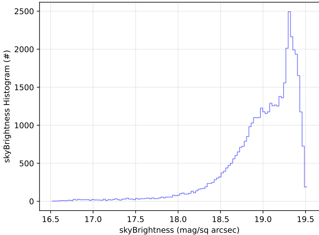
ddf_acor_sf10_lsf40_lsr20_v3.4_10yrs Yr 1 z band: skyBrightness Histogram
