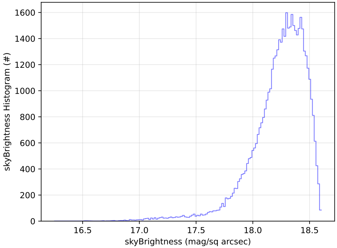
ddf_acor_sf10_lsf40_lsr20_v3.4_10yrs Yr 1 y band: skyBrightness Histogram
